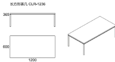
W1200*D600*H365
